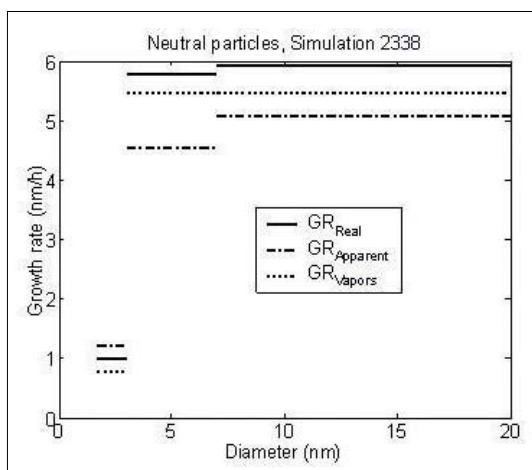
Figure 3. The growth rates of neutral particles as a function of particle diameter analysed from simulations carried out by ion-UHMA model. Different curves in the figure represent growth rates obtained 1) directly from model 2) by analysing method used for experimental data 3) directly from model input vapour concentrations.
